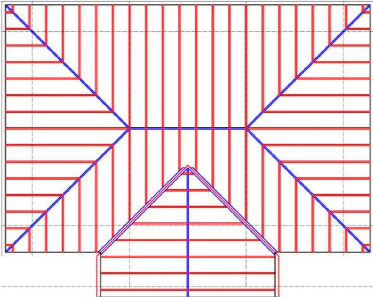
ROOF FRAMING (RAFTERS) STRUCTURE: (BATTENS/PURLING NOT SHOWN)
