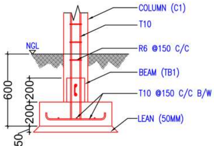
FOUNDATION DETAIL
